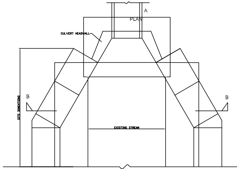
LAYOUT OF RETAINING WALL AT HEADWALL
