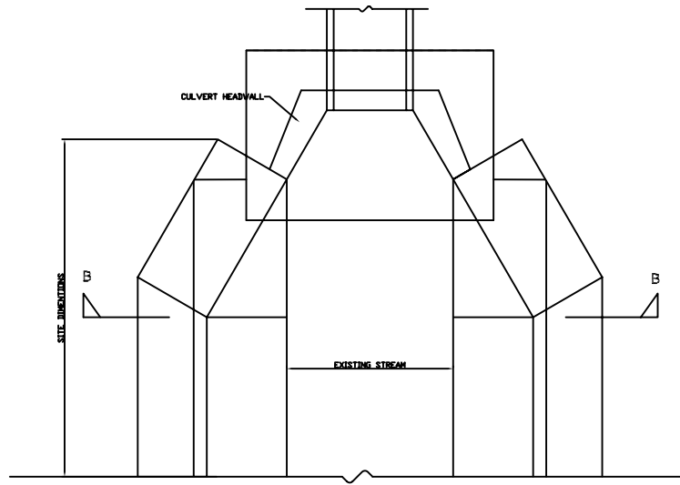
LAYOUT OF RETAINING WALL AT HEADWALL
