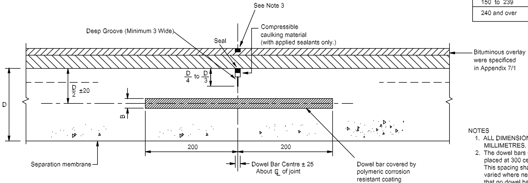
CONTRACTION JOINT - WITH SAWN GROOVE
